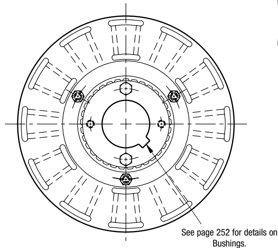
ARMATURE VIEW
