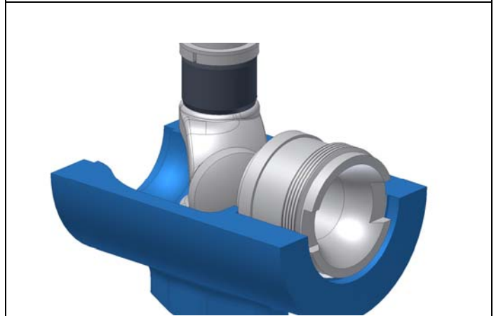
Fig. 4: Plug movement with double-eccentric arrangement
