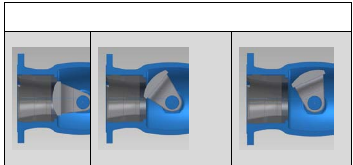
Fig. 3: Double-eccentric principle
