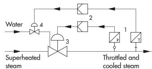
Fig. 1: Type 3286-1 Pneumatic Steam Converter
